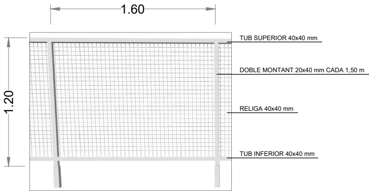
BARANA ACER COLOR NEGRE SE-03: BARANA INCLINADA: 9.60 ml x 1.20m BARANA RECTA (P2): 6.00 ml x 1.20m
